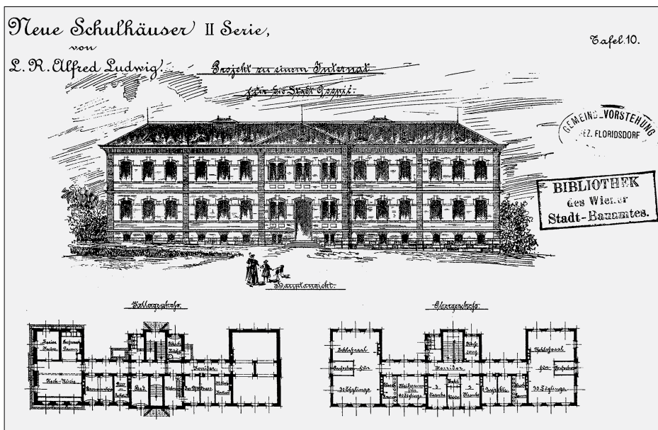
FIG. 19 LUDWIG & HÜLSSNER: DESIGN FOR THE BOARDING SCHOOL IN GOSPIĆ, 1894
