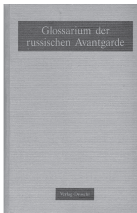
Prilog 2.
