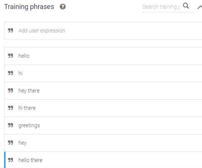
Slika 7: Training phrases
