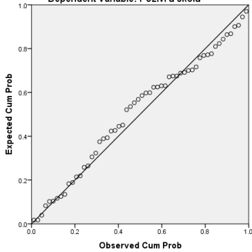
Normal P-P Plot of Regression Standardized Residual Dependent Variable: Pozivi u školu
