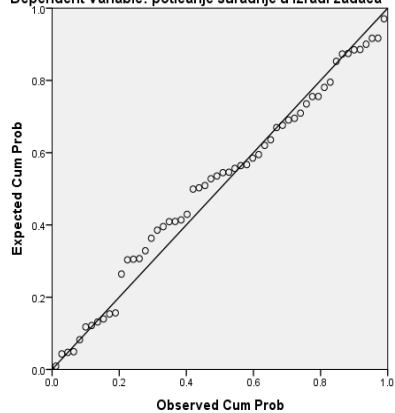
Normal P-P Plot of Regression Standardized Residual Dependent Variable: poticanje suradnje u izradi zadaća
