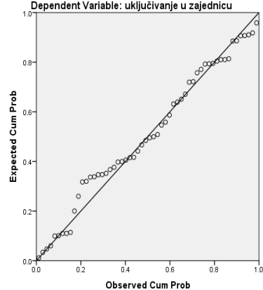
Normal P-P Plot of Regression Standardized Residual Dependent Variable: uključivanje u zajednicu
