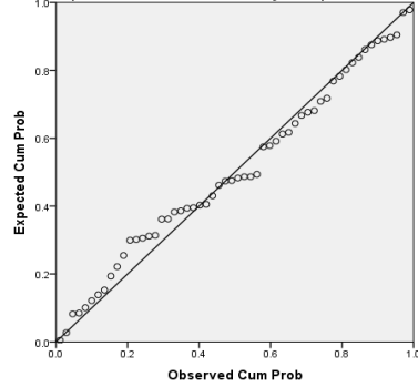
Normal P-P Plot of Regression Standardized Residual Dependent Variable: informiranje o napretku
