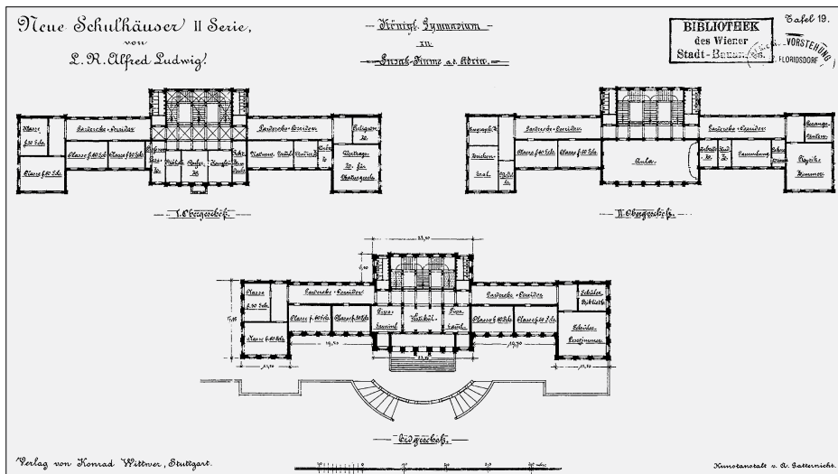
Sl. 8. LUDWIG & HÜLSSNER: TLOCRTI GIMNAZIJSKE ZGRADE NA SUŠAKU, 1894. FIG. 8 LUDWIG & HÜLSSNER: HIGH SCHOOL BUILDING IN SUŠAK, LAYOUT PLANS, 1894
